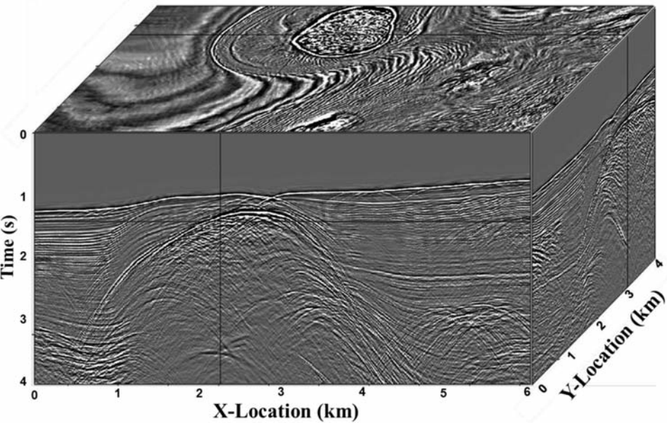
Fig. 3a. Quantum stacked cube.
